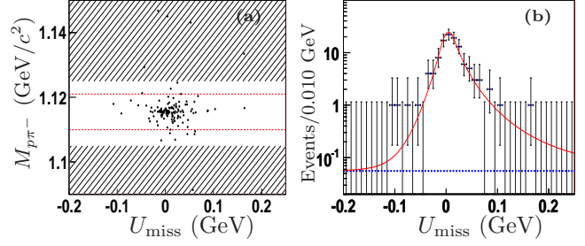
FIG. 2. (a) Scatter plot of M_{p\pi^-} versus U_{\text{miss}} for the \Lambda_c^+ \rightarrow \Lambda e^+\nu_e candidates. The area between the dashed lines denotes the \Lambda signal region and the hatched areas indicate the \Lambda sideband regions. (b) Fit to the U_{\text{miss}} distribution within the \Lambda signal region. The points with error bars are data, the (red) solid curve shows the total fit and the (blue) dashed curve is the background shape.
