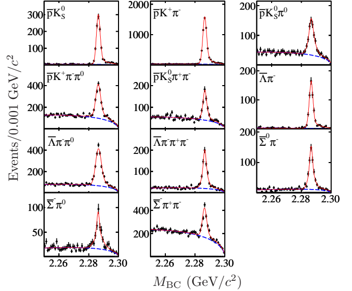
FIG. 1. Fits to the M_{\text{BC}} distributions for different ST modes. The points with error bars are data, the (red) solid curves show the total fits and the (blue) dashed curves are the background shapes.
